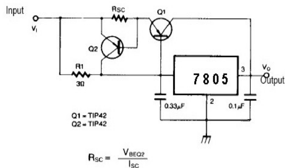
Figure 1. High Output Current with Short Circuit Protection
